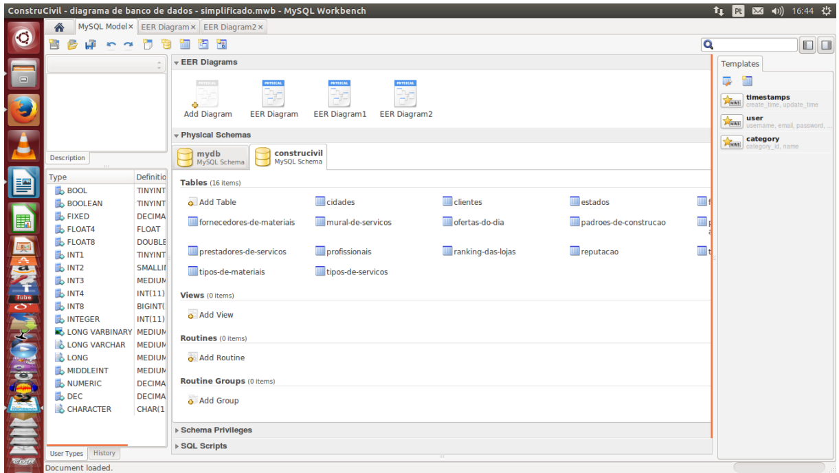
FIGURA 7: MYSQL WORKBENCH.
