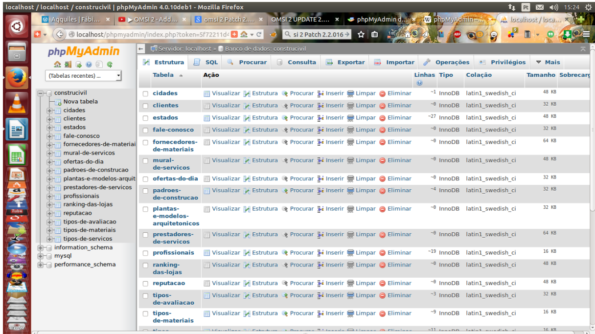
FIGURA 6: PHPMYADMIN.
