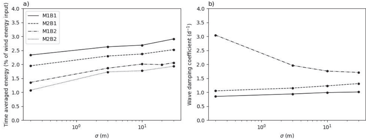
Figure 23 – Parameters related to wave generation and dissipation. a) Time averaged energy in internal seiches in response to a solitary wind event as a function of the initial density stratification (thermocline width \sigma , cf. Fig. 19) for the four simulated scenarios: M1B1, M2B1, M1B2, and M2B2. The line shows the initial wave energy computing assuming the energy from the first wave cycle. The internal seiche energy is normalized by the wind energy input. b) Wave damping coefficient obtained assuming an exponential decay of the total wave energy. Wave dampening of case M2B2 is not shown because the wave is rapidly dissipated right after the end of the wind event.
