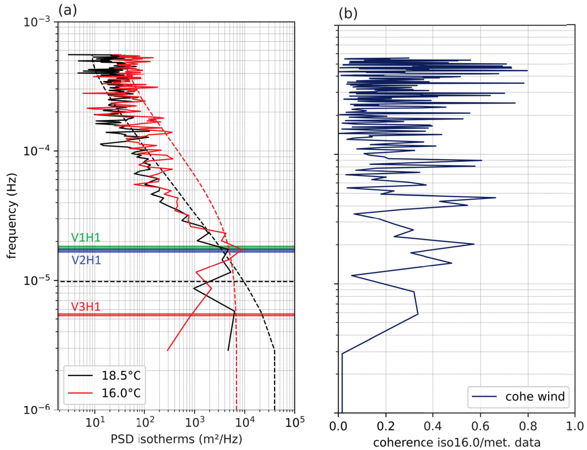
Figure 8 – Spectral analyses of Vossoroca reservoir during September 2012: a) Power spectral density of the isotherms of 18.5 °C and 16 °C (Vossoroca reservoir; 15/09 – 25/09). The dashed lines show the mean red noise spectrum for the time series, where spectral peaks above this line are significantly different from noise at a 95% confidence level. Horizontal color boxes indicate the theoretical period for different vertical modes. b) Coherence between 16 °C isotherm and wind speed.
