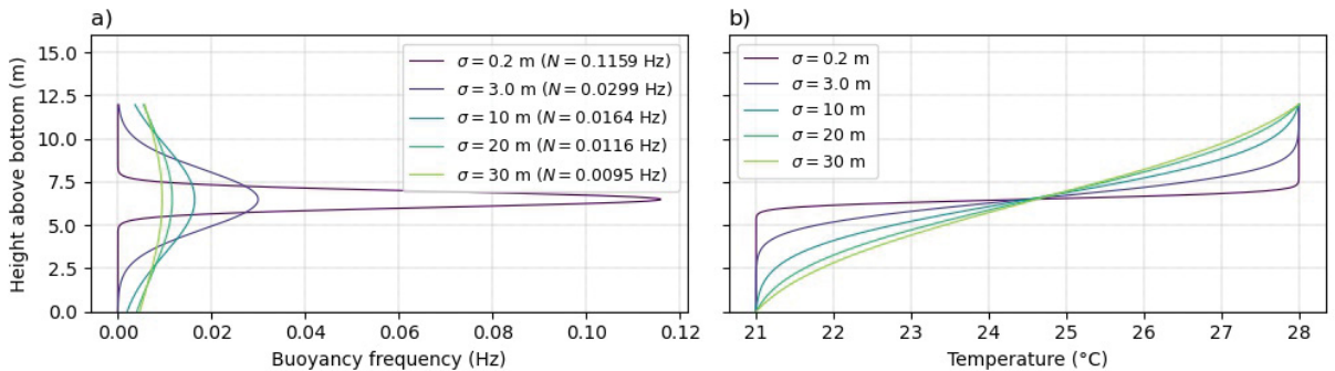
Figure 19 – Vertical profiles of density stratification used in the numerical simulations. a) Buoyancy-frequency ( N ) and b) temperature profiles for different values of \sigma (the standard deviation describing the Gaussian form of the buoyancy-frequency profile). N refers is the maximum buoyancy frequency of each stratification profile.
