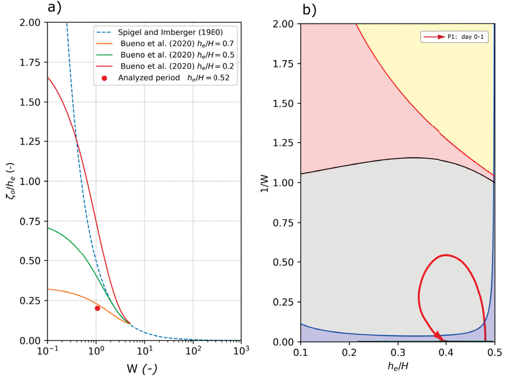
Figure 32 – a) Normalized internal wave amplitude (normalized by the epilimnion thickness ( \zeta_o/h_e )) versus Wedderburn number W . The blue solid line represents the theoretical formulation defined by Spigel and Imberger (1980), whilst green and yellow represent the empirical parameterization described by equation 4.10. The red dot indicates the maximum observed for the modeled wind event. b) Regime diagram characterizing the degeneration of basin-scale internal waves according to the theoretical classification (HORN; IMBERGER; IVEY, 2001). The variability of h_e/H and W marked by the red arrow refers to the first two days of simulation, which may characterize the degeneration regime of internal wave. The blue region indicates conditions when internal seiche are more susceptible to be damped by viscosity. The range colored in gray indicates a regime where internal waves degenerate into a propagating waves. The red and yellow region characterize regime of degeneration with formation of supercritical flow, and bore and billows, respectively.
