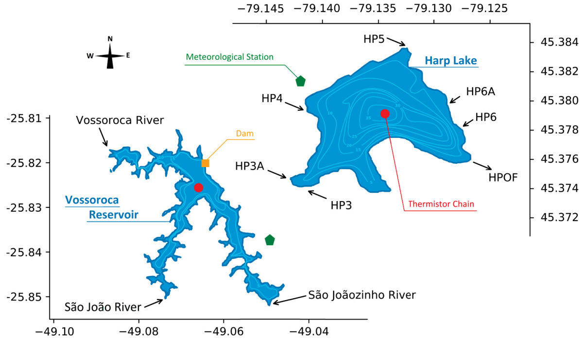
Figure 5 – Maps of Vossoroca reservoir (left), and Harp Lake (right), with depth contours and locations of observation points (green: meteorological station, red: platform with thermistor chain), and in and outflows (arrows).
