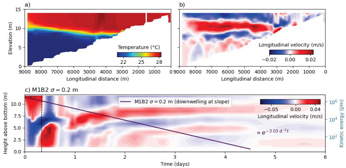
Figure 44 – The influence of bathymetry on internal seiches analyzed in scenario M1B2 (straight channel with sloping water depth) for nearly two-layer stratification ( \sigma = 0.2 m) in response to a wind event from southern direction (from the left towards the dam). a) Temperature distribution along the longitudinal cross section of the reservoir during the wind set-up ( t = 0.3 d) and b) the longitudinal flow velocity distribution at t \approx 38.5 h. c) Time series of horizontal velocity profiles at the basin center. The solid lines illustrate the exponential wave energy decay (see labels for decay rates, in which t is defined in days).
