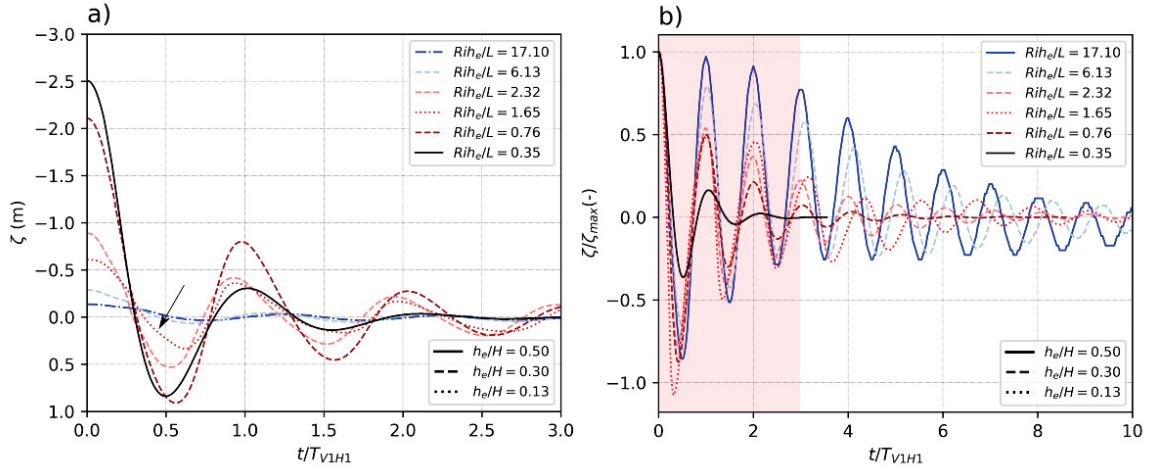
Figure 11 – Numerical simulations results: Evolution of the generated basin-scale internal waves. a) internal wave amplitude, and b) non-dimensional internal wave amplitude, plotted against the non-dimensional time (using the internal wave period T_{V1H1} for normalization) for different stratification conditions and pycnocline depths. The arrow indicates the anomaly of the run with h_e/H = 0.13 . The red region in b) indicates the same interval analyzed in a)
