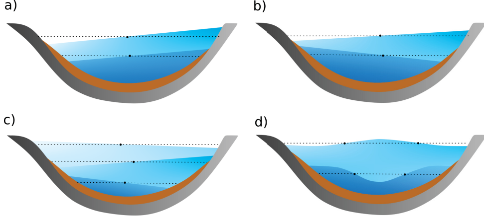
Figure 4 – Schematic view of various internal wave modes in a closed basin: a) V0H1, b) V1H1, c) V2H1 and d) V1H2. The mode for n = 0 is related to the pure surface (barotropic) mode. The black dots (·) represent nodal points
