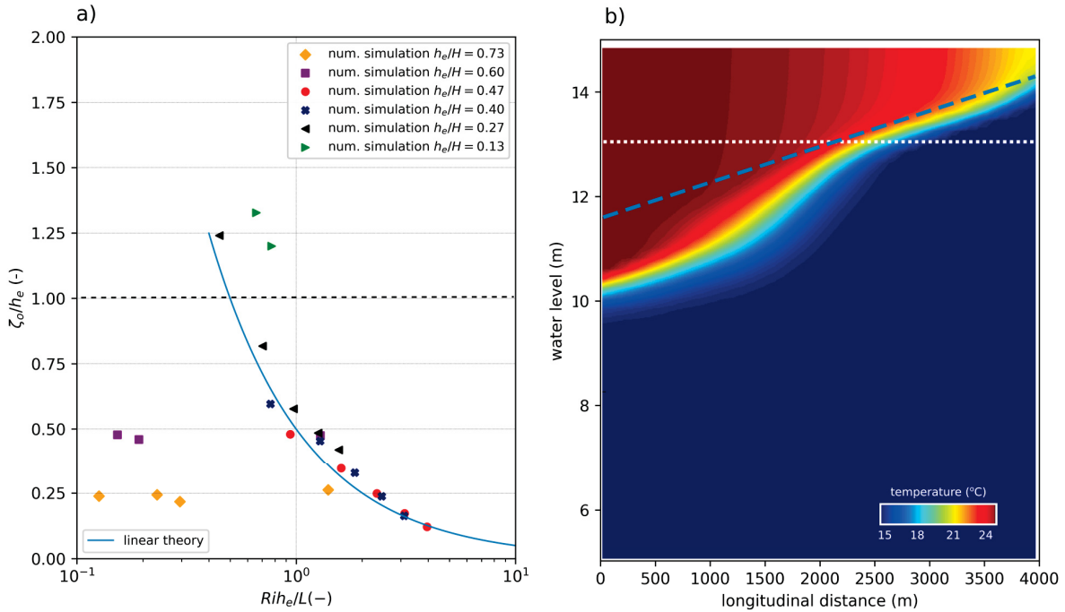
Figure 13 – a) Maximum basin-scale internal wave displacement normalized by the thermocline depth h_e at downwind regions, where the initial displacement is characterized by a downward movement. The horizontal dashed black curve indicates the limit boundaries to direct interaction between water surface and internal seiche at upwind region. b) The longitudinal temperature profile during the wind event (3 h of simulation time) showing the strong erosion of thermocline at downwind region (Simulation: Run 23). The white dashed line indicates the unperturbed thermocline depth and the blue dashed line the theoretical displacement according to linear theory.
