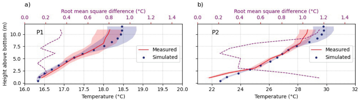
Figure 47 – Vertical stratification during the analysis periods at the sampling site near the intake station (Fig. 18a in the main text): a) P1 (from June 28 to July 04, 2018) and b) P2 (from January 29 to February 04, 2019). Both panels show the mean vertical profiles of simulated (blue dots) and measured (red solid line) temperature, with their standard deviations marked by the blue and red shaded areas. The purple dashed lines show the root mean square difference between simulations and observations.
