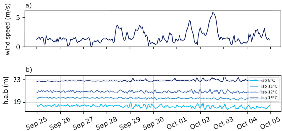
Figure 40 – Thermal and wind speed condition in Harp Lake. a) Wind speed time series (Harp Lake; 25/09 – 04/10). b) Isotherms time-series in height above the bottom (h.a.b.)
