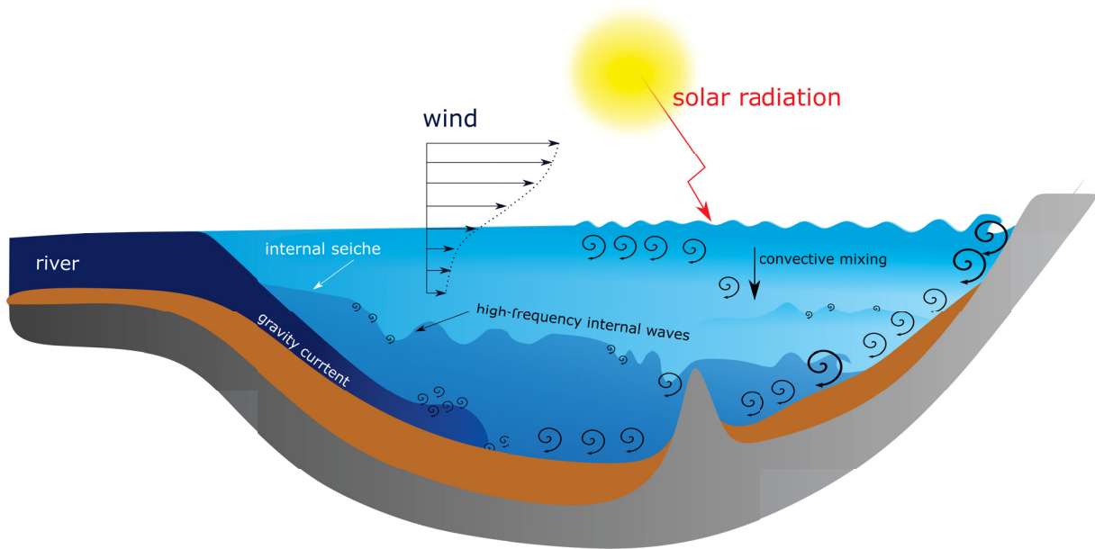
Figure 26 – Schematic overview of currents and mixing process in lakes and reservoirs. Different shades of blue denote layer of different temperature (density). Brown and silver layers indicate the sediment layer and the solid bathymetry of the lake, respectively. Basin-scale internal waves and high-frequency internal waves can occur at density interfaces. Billows (black arrows) illustrate turbulent mixing.
