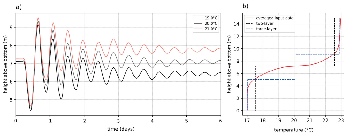
Figure 30 – a) Time series of selected isothermal depths at the sampling point ST in the numerical simulations. b) Temporally averaged vertical temperature profiles (red line) and the two (black line) and three-layer (blue line) approximation of the temperature profiles used for modal internal wave analysis.
