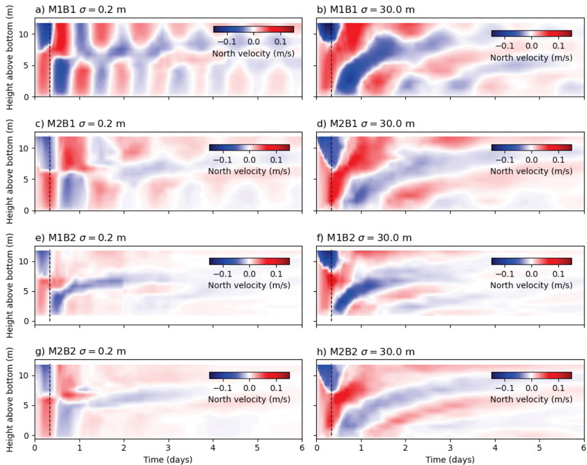
Figure 45 – Temporal dynamics of the vertical profiles of horizontal flow velocities near the center of the reservoir (station S1, velocity indicated by color) for scenario a) M1B1 \sigma = 0.2 m, b) M1B1 \sigma = 30 m, c) M2B1 \sigma = 0.2 m, d) M2B1 \sigma = 30 m, e) M1B2 \sigma = 0.2 m, f) M1B2 \sigma = 30 m, g) M2B2 \sigma = 0.2 m, and h) M2B2 \sigma = 30 m. The vertical black dashed lines mark the end of the wind event.
