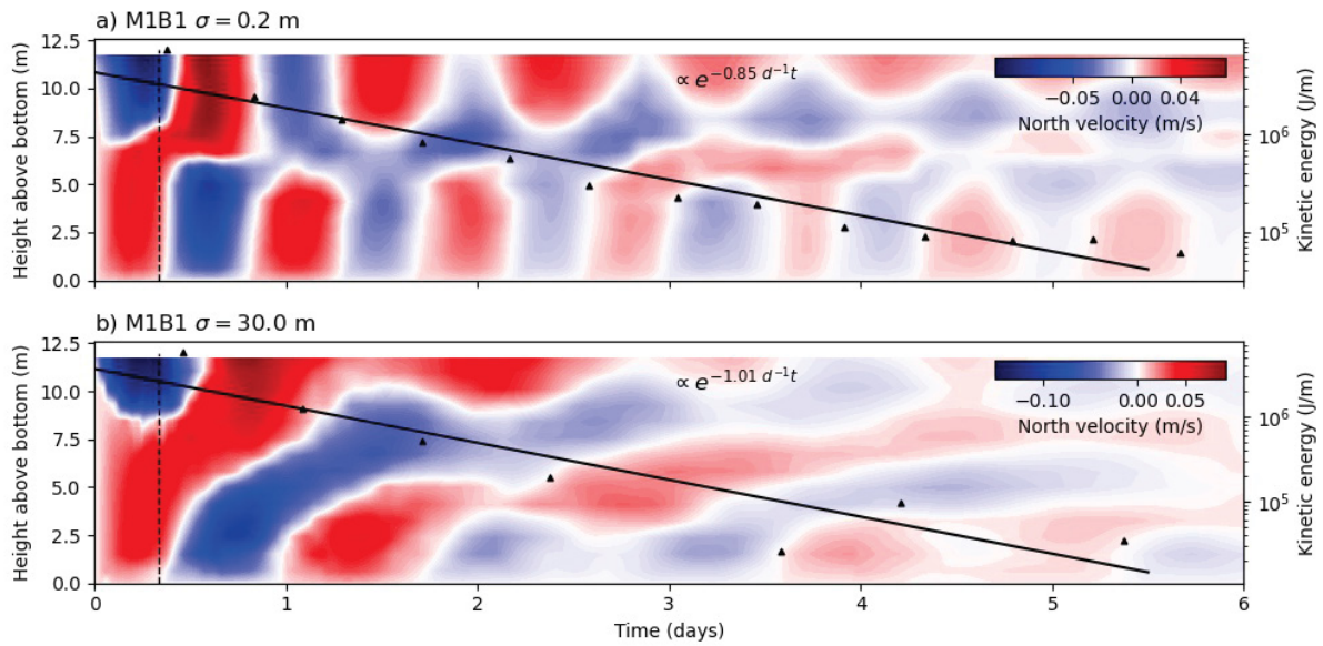
Figure 22 – Temporal dynamics of vertical profiles of horizontal flow velocities near the center of the reservoir (station S1, velocity indicated by color) and kinetic energy in internal wave motion for scenario M1B1 for a) nearly two-layer stratification ( \sigma = 0.2 m) and b) nearly linear stratification ( \sigma = 30 m). The vertical black dashed lines mark the end of the wind event. The black triangles show the total internal wave energy. The black solid line illustrates the exponential decay of wave energy (see labels for decay rate, in which the time t has the unit days).
