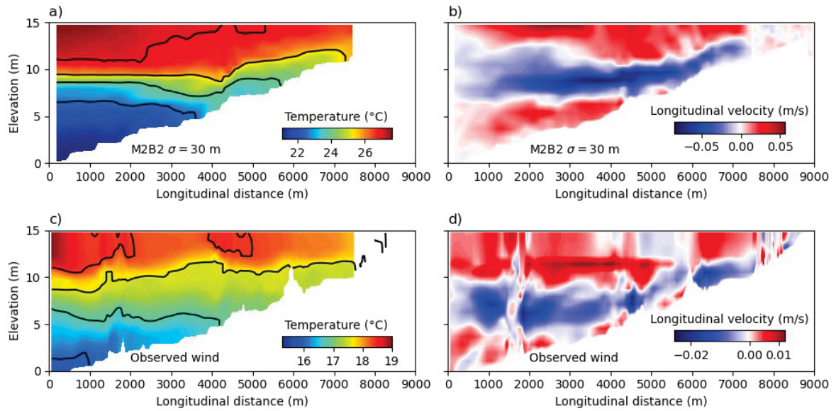
Figure 42 – Longitudinal sections of water temperature and horizontal flow velocity in Passauna Reservoir in response to an idealized 8-h wind episode (scenario M2B2) and with observed wind forcing. a) Water temperature and b) longitudinal flow velocity for scenario M2B2. c) Water temperature and d) longitudinal flow velocity simulated with observed wind dynamics and measured initial water temperature profile. The temperature distribution was obtained at the end of the wind episode, which was at t = 8 h in a), while for the measured data the end of the wind episode was characterized by the end of a strong wind event measured on 29 June at 21 h 20 min (cf. Fig. 20 in the main text). The horizontal velocities are shown at the end of the wind event, during the initial seiche excitation. The solid black lines in a) and c) mark isothermal depth with 1.0 °C increment.
