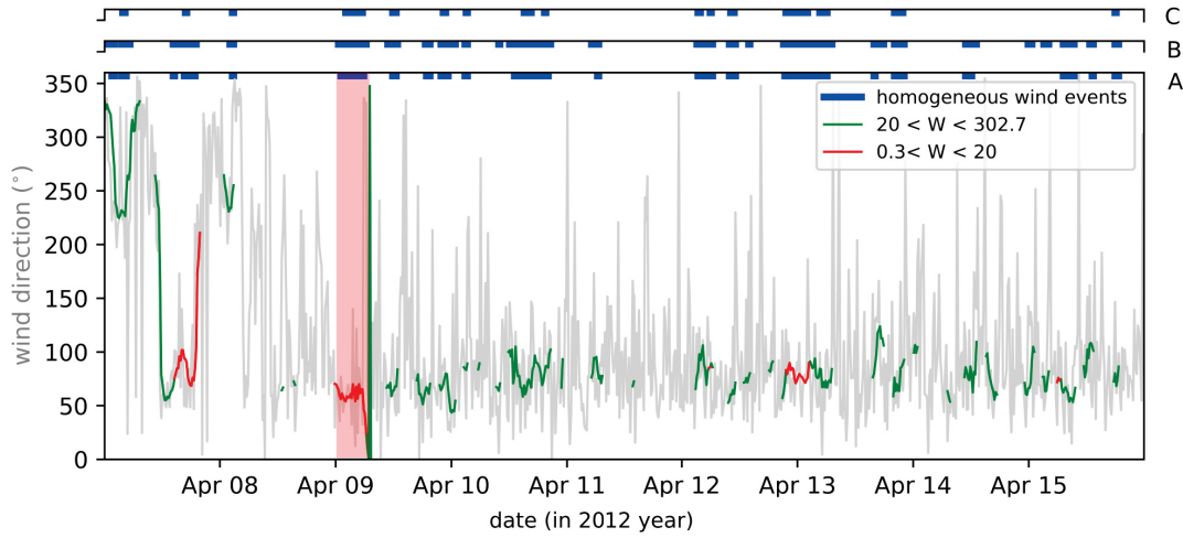
Figure 35 – Time series of wind direction at Vossoroca reservoir (grey line). The blue bars above the graph indicates periods of constant wind directions according to three different angles of wind direction contribution: A: \pm 20^\circ , B: \pm 40^\circ , and C: \pm 5^\circ . Periods marked by green and red color correspond to criteria suggesting internal wave generation. The green line represents the more flexible criteria often described by mathematical results from Spiegel and Imberger (1980). The red line indicates a more restrictive result, which fall into regime of internal wave described by Spiegel and Imberger (1980) and often observed from field data reported in the wide literature. The value of W_{V1} displayed in the label indicates an average for the entire period, and just illustrates the mean value of the adopted criteria. The vertical red bar indicates the period in which the internal wave was generated.
