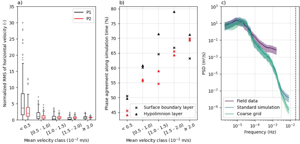
Figure 48 – Comparison of measured and simulated horizontal flow velocities for period P1 (weaker stratification) and P2 (stronger stratification). a) Normalized root mean square difference (NRMSD) of the horizontal velocity difference between measured and simulated data for different velocity classes for period P1 (black) and P2 (red). The boxes extend over the 25th and 75th quartiles, whilst the horizontal line indicates the median value. The whiskers extend to the minimum and maximum values neglecting outliers, which are represented by gray dots. b) Period of time (in percentage) that the direction of simulated horizontal velocities agreed with measured data for both periods and for different velocity classes. Crosses and triangles represent data from near the reservoir bottom (2.5 m above the bottom) and near the water surface (9 m above the bottom), respectively. c) Power spectral density of horizontal velocity variations at approximately 2.5 m above the bottom for measured (purple) and two simulations (blue and green). The solid blue line represents the spectral density of simulations using the standard grid size of our scenario analyses, whilst the solid green line represents PSD obtained from a coarser numerical grid. The colored shaded area shows the 95% confidence interval.
