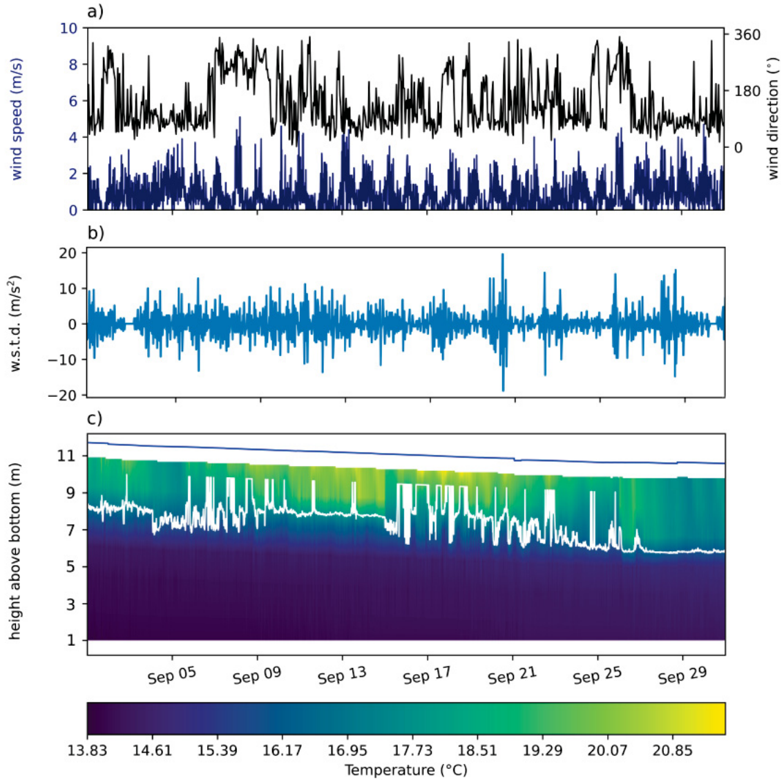
Figure 7 – Overview of field data from Vossoroca reservoir during September 2012 (Vossoroca reservoir; 01/09 – 29/09). a) Wind speed and direction, b) wind change with time, and c) thermal structure showing temperatures in colors and the thermocline position as a white solid line. The water surface elevation is represented by the blue solid line.
