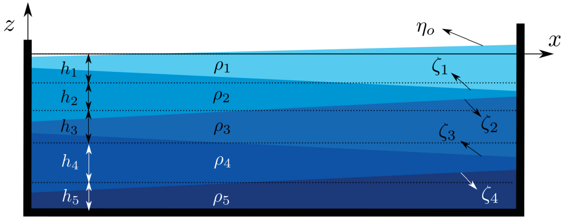
Figure 27 – Illustration of the modal structure of basin-scale (standing) internal waves in an idealized (rectangular) basin. Vertical density stratification is approximated by five vertical layers, (different shades of blue), each having a constant density \rho and thickness (at equilibrium position h ). The equilibrium position of the layer interfaces is shown as black dashed lines. The blue shading illustrates the layer displacement ( \zeta ) of a horizontal mode 1 and vertical mode four wave (V4H1). \eta_o denotes the displacement of the water surface.
