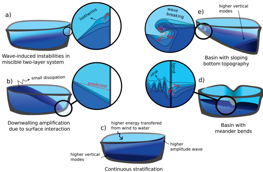
Figure 38 – Summary of the main findings related to the mechanism of wave dissipation observed during upwelling events and internal seiche activity. Explanations are provided in the text.
