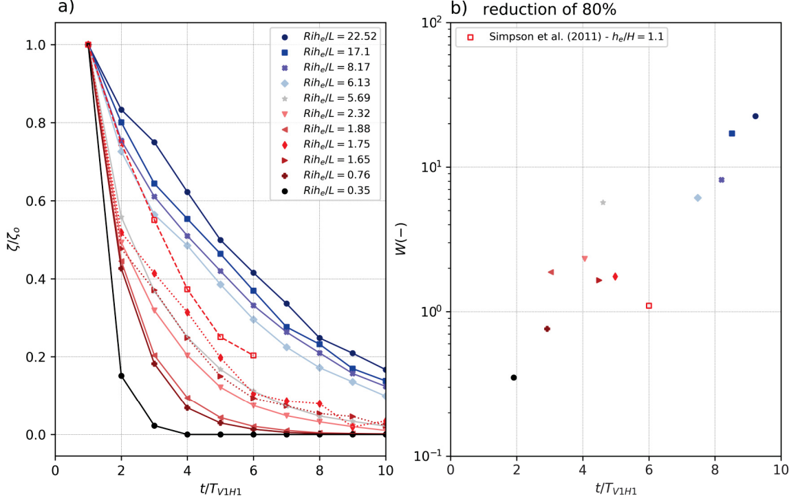
Figure 12 – Numerical simulations results: Initial displacement of the generated basin-scale internal waves. a) Decay of the non-dimensional internal seiche amplitude (using the initial displacement for normalization) as a function of the non-dimensional time (using the internal wave period T_{V1H1} for normalization). b) Ri\ h_e/L as a function of non-dimensional time in which 80% of internal wave energy is dissipated.
