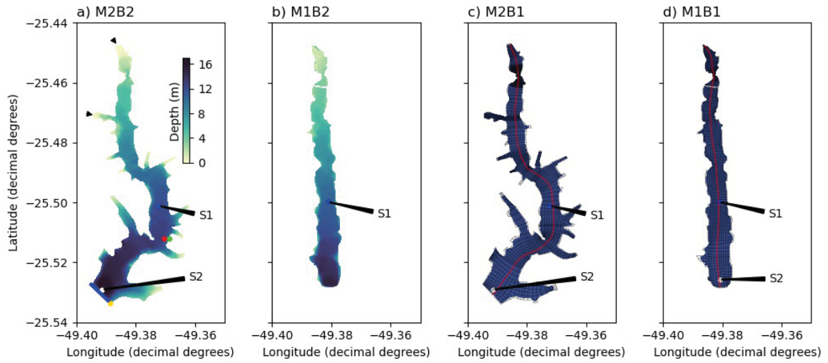
Figure 18 – Bathymetric maps of Passaúna reservoir and of the hypothetical basins considered in numerical simulations (the color map represents water depth). a) Scenario M2B2: Original shape (morphology, M) and bathymetry (B) of Passaúna reservoir. b) Scenario M1B2: Simplified (straightened) reservoir shape with similar bathymetry as the original reservoir. c) Scenario M2B1: original reservoir shape, but with constant water depth. d) Scenario M1B1: Simplified reservoir shape with constant depth. The black lines in c) and d) show the grid used for the numerical simulations. The red line marks the longitudinal grid positions for which the horizontal flow velocity in the north/south direction is illustrated in Fig. 25. The red, yellow, and green dots in panel a) show the location of the monitoring station, the weather station, and the reservoir intake, respectively. Small triangles show the inflows, and the blue line indicates the location of the reservoir dam. The stations S1 and S2 (blue and white symbols) are used in the discussion of the numerical simulations.
