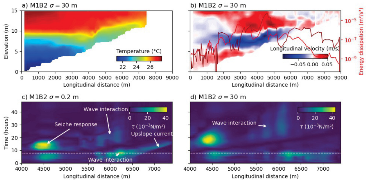
Figure 46 – Simulated water temperature, horizontal flow velocity, bed shear stress, and depth-integrated energy dissipation rates at the center line of Passaúna reservoir for scenario M1B2. a) Longitudinal cross section of water temperature (at t = 7 h 12 min) and b) horizontal velocity (at t = 7 h 12 min). Light and dark red lines show time series of integrated turbulent energy dissipation rates during the first interaction with the lakeshore for scenario M1B1 with \sigma = 0.2 m and \sigma = 30 m, respectively. Bed shear stress for c) \sigma = 0.2 m and d) \sigma = 30 m at the center line of Passaúna reservoir. High shear stress observed after the wind event (above the dashed white line) at the center of the basin (4500 m from the dam) indicates the response of internal seiche, since higher horizontal velocity are observed near the wave node (seiche response). Right after the end of the wind event high shear stress is observed near the shore, where the current shear across the density interface interacts with the bottom slope, at 6200 m from the dam (wave interaction). This occurs due to the acceleration of the flow near the sloping bottom, causing a up sloping current. This event persists for more wave periods (wave interaction) but promoting lower shear stresses since most part of the energy has been dissipated during the first interaction.
