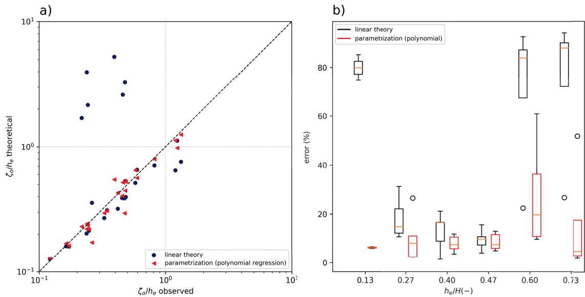
Figure 15 – a) Comparison between theoretical (linear and parametrized equation) and internal seiche amplitude detected in simulations. b) Error percentage with respect to h_e/H .
