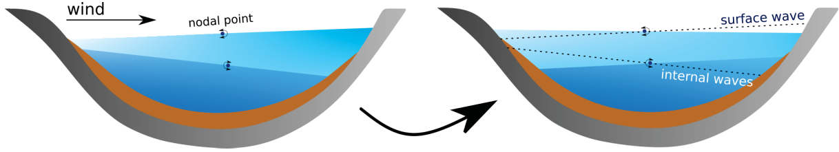
Figure 3 – A wind-induced stationary internal wave in a stratified basin. Left: Tilting of surface and interface, due to wind stress. Right: Oscillatory motion of surface and interface after wind stopped at one half of the wave period. Dashed lines indicate surface and interface location right after wind stopped.
