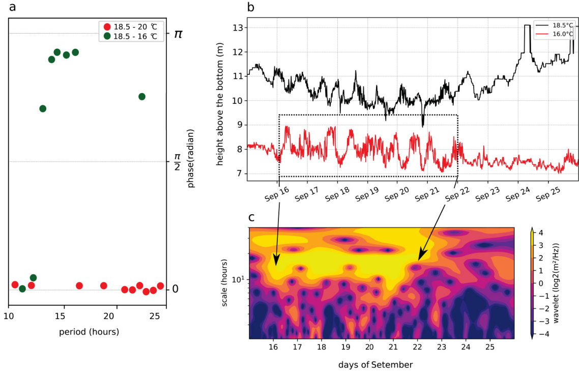
Figure 9 – Isotherm, phase, and wavelet analyses of Vossoroca reservoir during September 2012. a) Phase analyses of two pairs of isotherms (phase was just plotted for coherence above the 95% confidence level). b) 16 °C and 18.5 °C isotherm time series. c) Wavelet analyses of the 16 °C isotherm (Vossoroca reservoir; 15/09 – 25/09)
