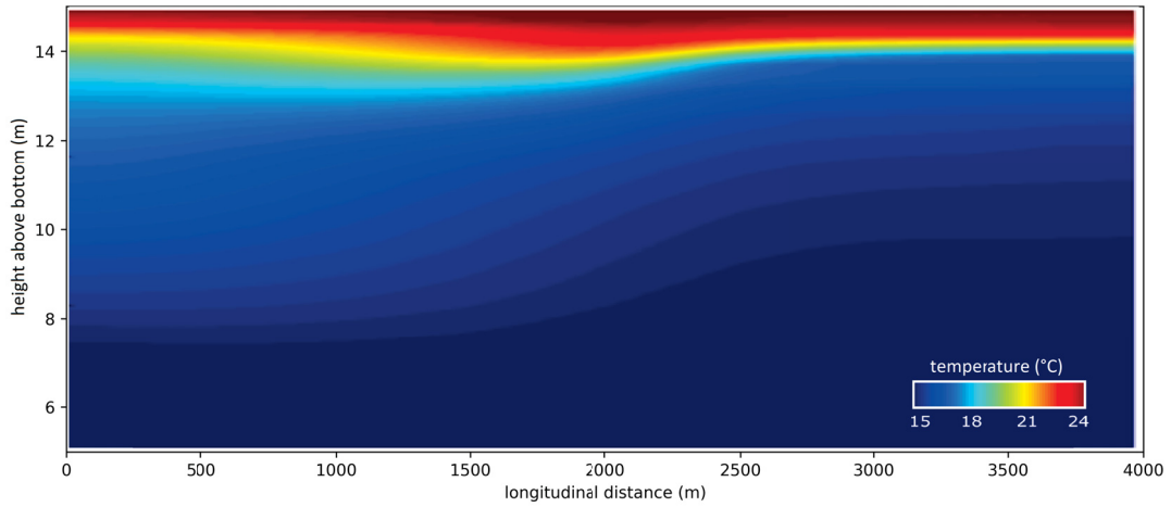
Figure 39 – Internal bore generated as a result of the degeneration process of basin-scale internal wave (Simulation: Run 23)
