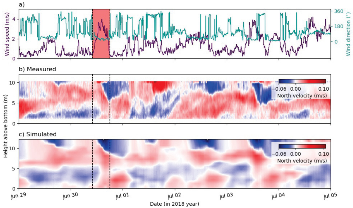
Figure 21 – a) Wind speed (purple line) and wind direction (green line) during the analysis period P1. The red shaded area, delimited by vertical black dashed lines, marks a solitary wind event that may favor the generation of internal seiches. b) Measured, and c) simulated horizontal flow velocities in south to north direction at the location of the monitoring station (Fig. 18a) with a temporal resolution of 1 min.
