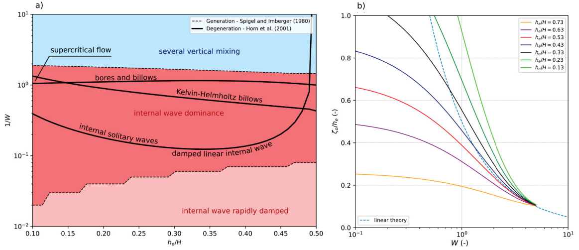
Figure 28 – a) Regime diagram for generation and degeneration of internal waves for a hypothetical reservoir with a basin length of L = 4 km. Different colors separate three mixing regimes based on Wedderburn number W_{V1} and the epilimnion thickness ( h_e ) normalized by the lake depth H . The two regimes proposed by Spigel and Imberger (1980), which result in complete vertical mixing are combined in the severe vertical mixing . Dashed lines show regime boundaries according to Spigel and Imberger (1980). Solid lines separate regimes of wave degeneration, as proposed by Horn, Imberger and Ivey (2001). b) The theoretical relationship between W_{V1} and the vertical displacement of the thermocline \zeta_o normalized by the epilimnion thickness ( h_e ). Solid lines show theoretical results from Spigel and Imberger (1980) and the dashed line shows the empirical formulation proposed by Bueno et al. (2020). The latter takes an additional contribution of the epilimnion thickness and the interaction of the internal seiche with the lake boundaries into account.
