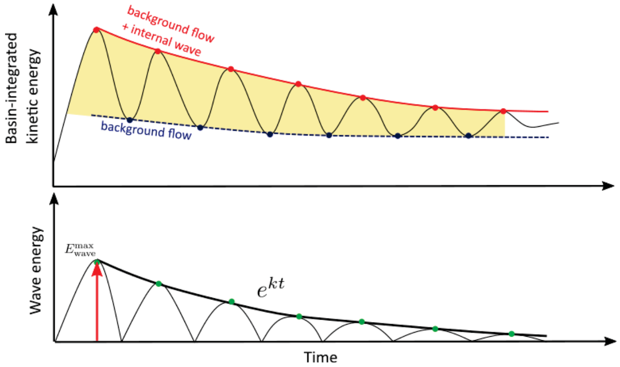
Figure 50 – Time-series of internal wave energy ( E_{\text{wave}} ) and the procedure to remove the background flow from the basin-integrated kinetic energy (Eq. 3.2 in the main text). Red and blue dots represent the identified maximum and minimum values from the time-series of basin-integrated kinetic energy, respectively. Red solid and blue dashed lines represent the total energy decay and the background flow decay, respectively. Green blue dot is the internal wave energy obtained from the difference between the basin-integrated kinetic energy (red dots) and the function of the background flow energy (blue dashed line), in which the first green dot (red arrow) describes the initial energy of the internal wave ( E_{\text{wave}}^{\text{max}} ). k is the internal wave damping coefficient (Eq. 3.3 in the main text).
