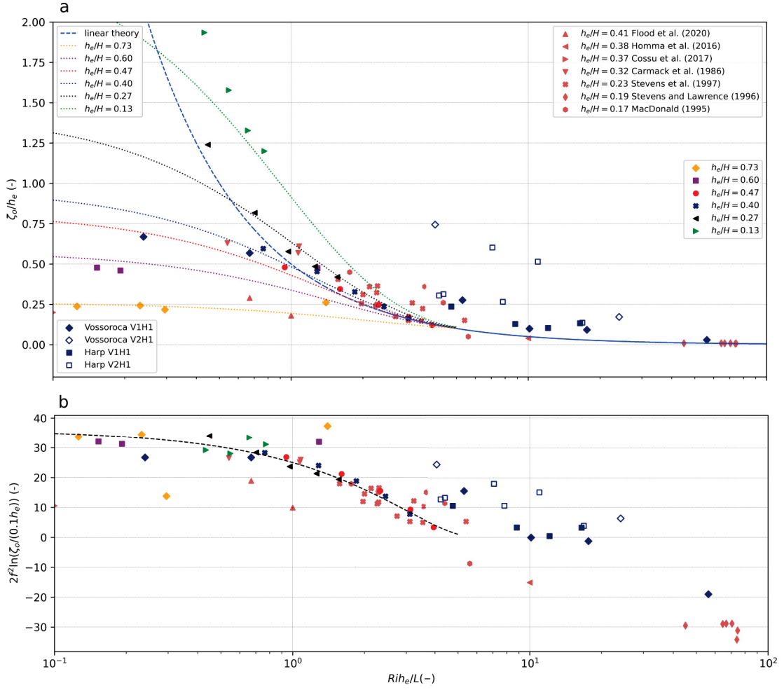
Figure 16 – a) Maximum vertical displacement associated with internal seiche normalized by the epilimnion thickness against Ri h_e/L . Data points include values from simulations, Harp lake, Vossoroca reservoir, and many other lakes from the literature (FLOOD et al., 2020; HOMMA et al., 2016; COSSU et al., 2017; CARMACK et al., 1986; STEVENS; LAWRENCE, 1997; STEVENS et al., 1996; MACDONALD, 1995) b) Normalization of \zeta_0/h_e to incorporate the function f(h_e/H) ( 2 f^2 ) against Ri h_e/L . The black dashed line represents Eq. 2.8 normalized by 2 f^2 . "Log" is defined in base e, natural logarithm.
