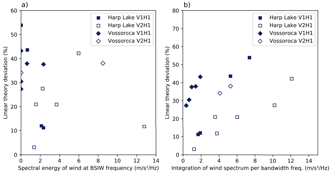
Figure 17 – Amplitude growth due to resonance effect against a) the peak of the power spectral density of the wind intensity at the internal seiche period and b) the integration of the wind spectrum for wind frequencies between 0.5 to 1.5 of the internal wave period per bandwidth frequency.
