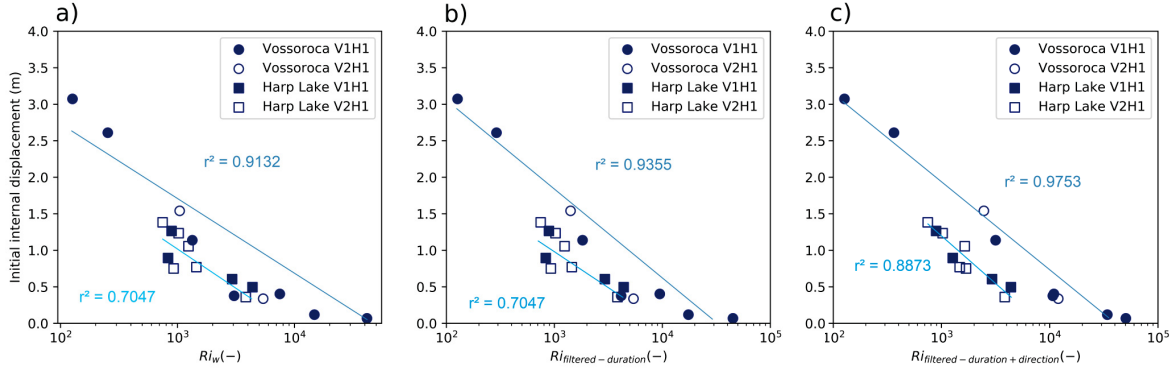
Figure 10 – Internal seiche amplitude of the most energetic isotherm versus a) the daily Ri , b) filtered Ri_{\text{duration}} using only periods with winds capable to generate internal waves, and c) filtered Ri_{\text{direction}} using only periods with winds in directions capable to generate internal waves. Linear regression was obtained for each basin
