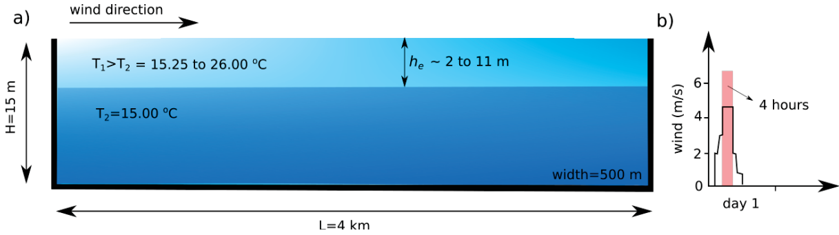
Figure 6 – a) Sketch of the numerical experiment and b) the wind event responsible to excite a BSIW for all numerical simulations. Red bar indicates the period of homogeneous wind.
