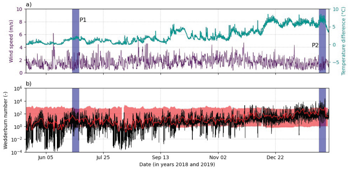
Figure 20 – Conditions at Passaúna reservoir during the monitoring period. a) 3-h average wind speed measured at the meteorological station near the dam (purple solid line) and temperature difference between the water surface and the bottom (green solid line). b) Wedderburn number ( W ) calculated with 3-h resolution (black solid line) and averaged over one internal seiche period (red solid line). The red background color marks the range of W , for which internal seiche dominance is predicted by a common classification scheme (Fig. 49). The vertical blue bars indicate the two analysis periods (P1, from June 28 to July 04), and P2 (from January 29 to February 04).
