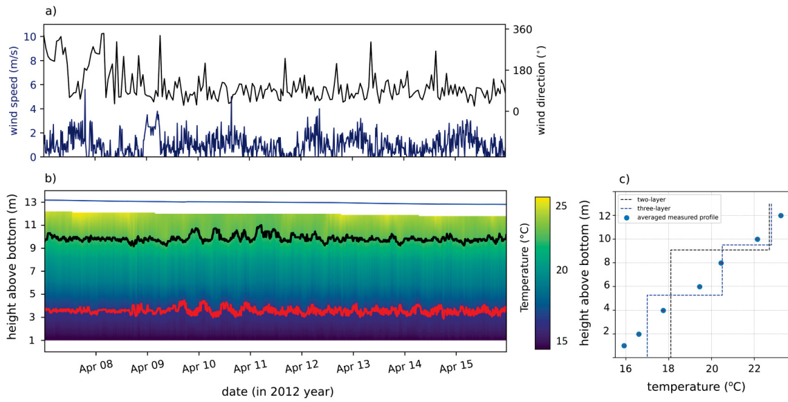
Figure 34 – Measurements at Vossoroca reservoir: a) Wind speed and direction. b) Water temperature measured by a thermistor chain. The solid blue line represents the water surface. black and red lines represent the isotherms of 22 °C and 17.5 °C, respectively. The altitude of reference for reservoir bottom is 799 m. c) Temperature profile estimated by the software for a two- and three-layer approximations. The blue dots show the mean temperature measured by the 7 thermistors deployed in the reservoir.
