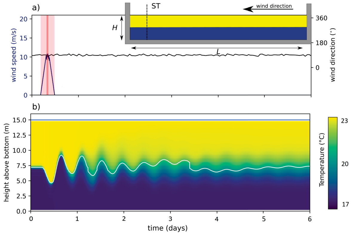
Figure 29 – Results of the numerical simulation of water temperature in an idealized (rectangular) basin in response to a single wind event. a) Time series of wind speed (blue solid line) and wind direction (gray solid line). The dark and light vertical red box indicates the period of maximum and the total duration of the wind event, respectively. The inset figure shows a sketch of the two-layer rectangular tank of H = 15 m and L = 4.5 km with the initial temperature distribution. ST is the location where temperature time series were analyzed. b) Contour plot of water temperature at station ST. The solid blue and white line represent the water level ( H = 15 m) and the thermocline, respectively.
