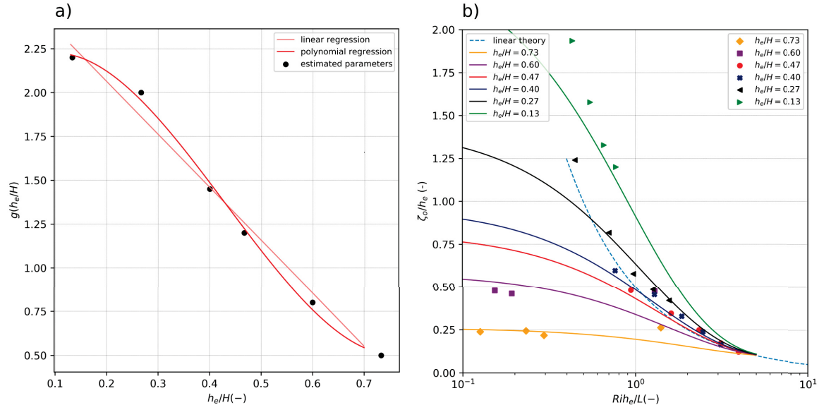
Figure 14 – a) Variation of g as a function of h_e/H for all simulated cases. Black dots represent the empirical parameter defined considering all simulated h_e/H condition. Red curves indicate different functions to describe the variability of g(h_e/H) (linear and a third order polynomial regressions). b) Maximum vertical displacement associated with internal seiche. Solid curve is derived from parametrized equation (Eq. 2.8) for different h_e/H conditions applying the third-order polynomial equation to describe the g function, expressed with distinct colors. The result using the linear equation for g is presented in Appendix A. Marks indicate the simulated results from different h_e/H conditions.
