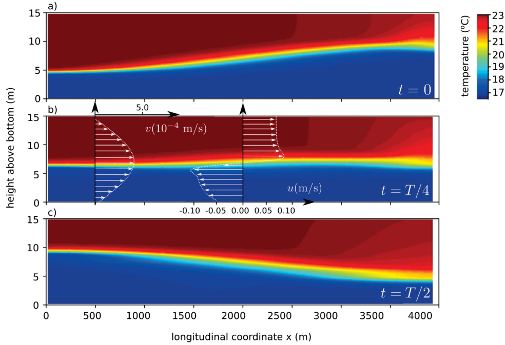
Figure 33 – Overview of the water temperature distribution along the centerline of the rectangular basin for three selected times: a) right after the wind event ( t=0 ), b) t = T_{V1H1}/4 , and c) t = T_{V1H1}/2 , in which T_{V1H1} is the theoretical period of the fundamental basin-scale internal wave. The vertical ( v ) and horizontal ( u ) velocity profiles are shown at different locations near the basin shore and in the center of the reservoir ( x \approx 2000 m), respectively.
