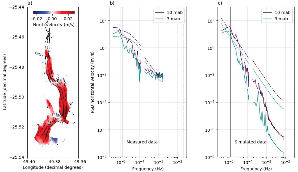
Figure 43 – Hydrodynamic characterization of the analyzed period P1. a) Simulated horizontal flow velocity during the upwelling event on June 29 (2018) at 17 : 00 h. The black arrows illustrate the horizontal velocity direction and magnitude near the water surface (2 m depth). The color scaling shows opposing (northward) flow in the hypolimnion (8 m above the deepest part of the reservoir). Power spectral density of b) observed, and c) simulated time series of horizontal flow velocity at two different depths at the monitoring station (red dot in Fig. 18a in the main text). For low-frequencies ( 10^{-6} to 10^{-4} Hz), the spectra were calculated with a window size of 3 d, while in the high-frequency range (up to 10^{-4} Hz), we used a window size of 12 h. The dashed lines show the 95% confidence limit of the mean red noise spectrum estimated for each time series. The vertical black dashed line marks the buoyancy frequency ( N = 0.02 Hz), and the vertical solid black line shows a 24-h period.
