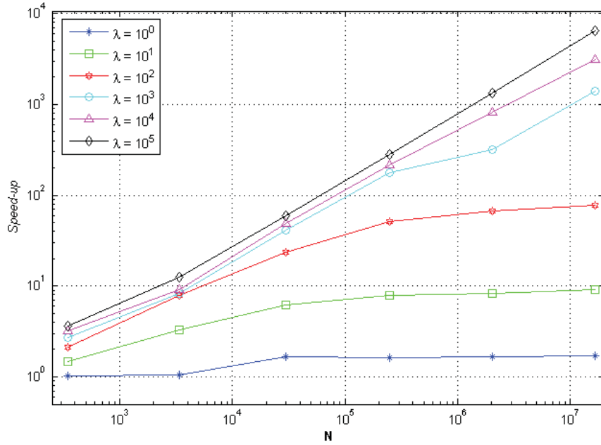
FIGURA 39 – SPEED-UP VERSUS N COM TIME-STEPPING - 2D.
