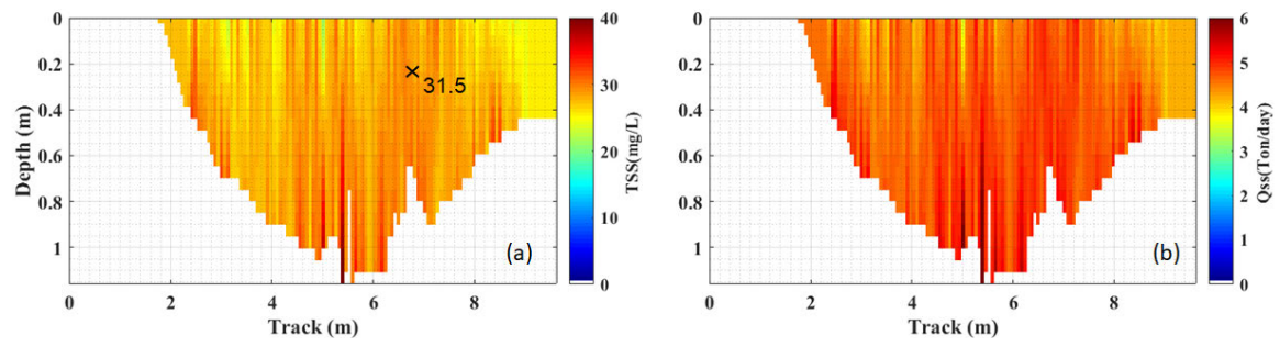
Figure 67 – Mapped cross-section in 20Oct/18 (a) TSS, (b)Qss.
