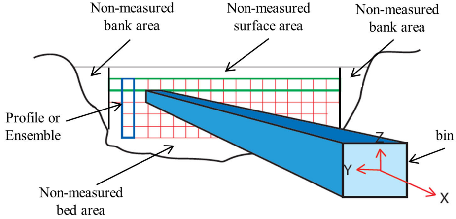
Figure 11 – Measured Area and Cross-Section component.
