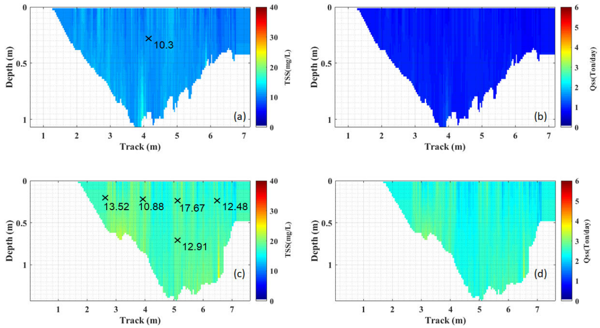
Figure 65 – Mapped cross-section in May/17 (a) TSS, (b)Qss and in Apr/18 (c) TSS, (d) Qss.
