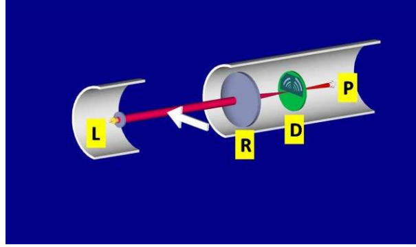
Figure 12 – Operating scheme of LISST equipment series - diffraction laser.
