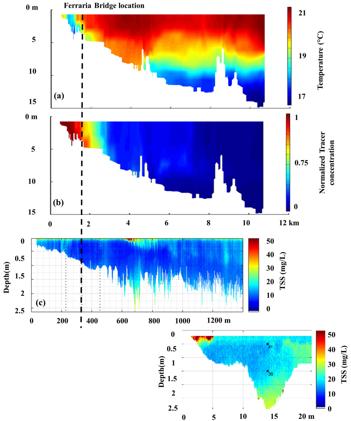
Figure 55 – Comparisons of the measurements performed on 20Oct/18 among numerical modeling for (a) Temperature and (b) Tracer Normalized Concentration (courtesy from Wendy Gonzales) the mapped longitudinal transect and (d) the mapped cross-section made with the ADCP, both already discussed at Figure 51.
