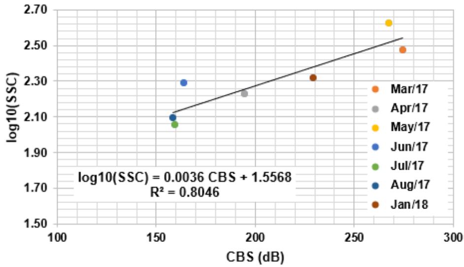
Figure 36 – Correlation curve between SSC and ADCP corrected backscatter signal (CBS) at Taquari River.
