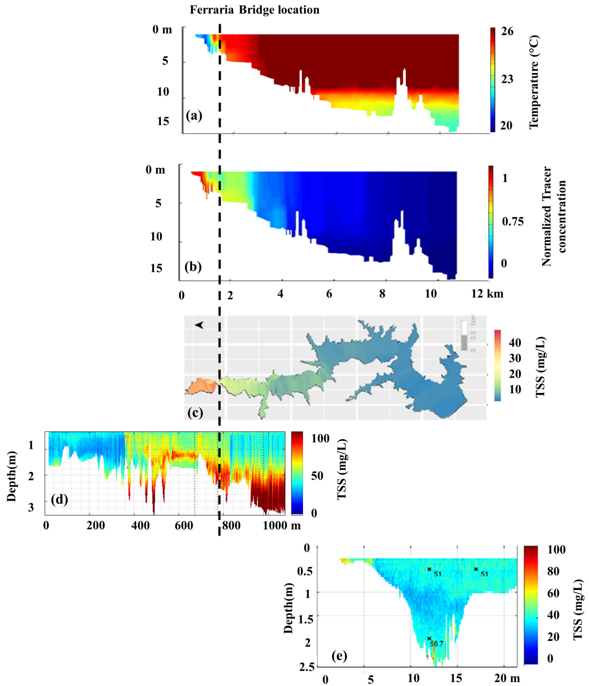
Figure 57 – Comparisons of the measurements performed on 05Feb/19 among numerical modeling for (a) Temperature and (b) Tracer Normalized Concentration (courtesy from Wendy Gonzales), (c) the TSS in the water surface obtained by close remote sensing, after Wagner (2019) , (d) the mapped longitudinal transect and (e) the mapped cross-section made with the ADCP, both already discussed at Figure 52.
