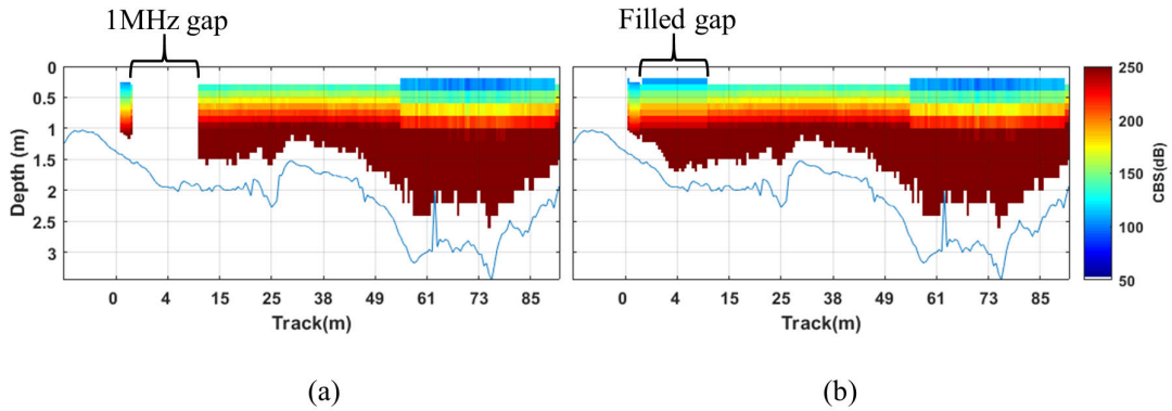
Figure 37 – Measured ADCP signal in the cross-section: (a) without the 1MHz measured cells and (b) with the 1MHz cells filled with the extrapolations obtained by the average of the signal measured by the 3MHz cells.
