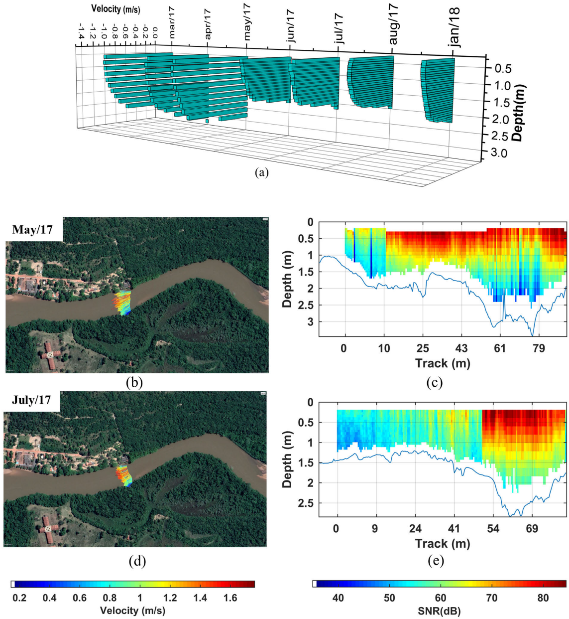
Figure 33 – (a) Mean velocity profiles during all measurement campaigns, Horizontal velocities during the measurement campaigns of (b) May/17 and (d) July/17 and Mean Backscatter Signal obtained during the measurement campaigns of (c) May/17 and (e) July/17.
