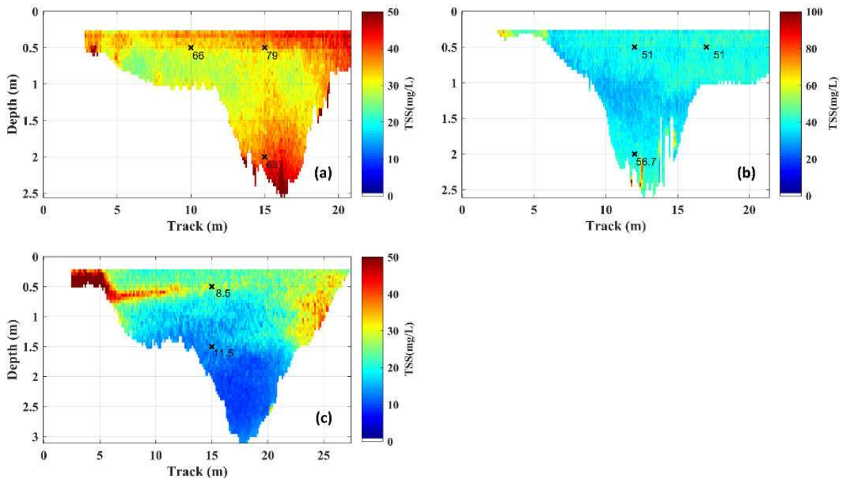
Figure 69 – Mapped cross-section in (a) 04Feb/19, (b) 05Feb/19 and (c) Apr/19.
