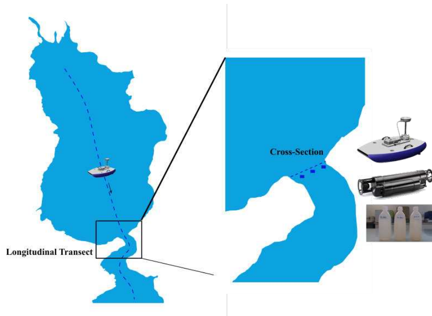
Figure 25 – Longitudinal Transect and Cross-section sketch at Passauna Reservoir.
