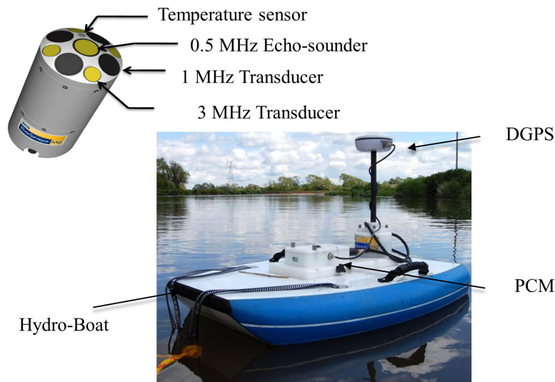
Figure 26 – ADP-M9 features. Adapted from: Sontek (2016) .
