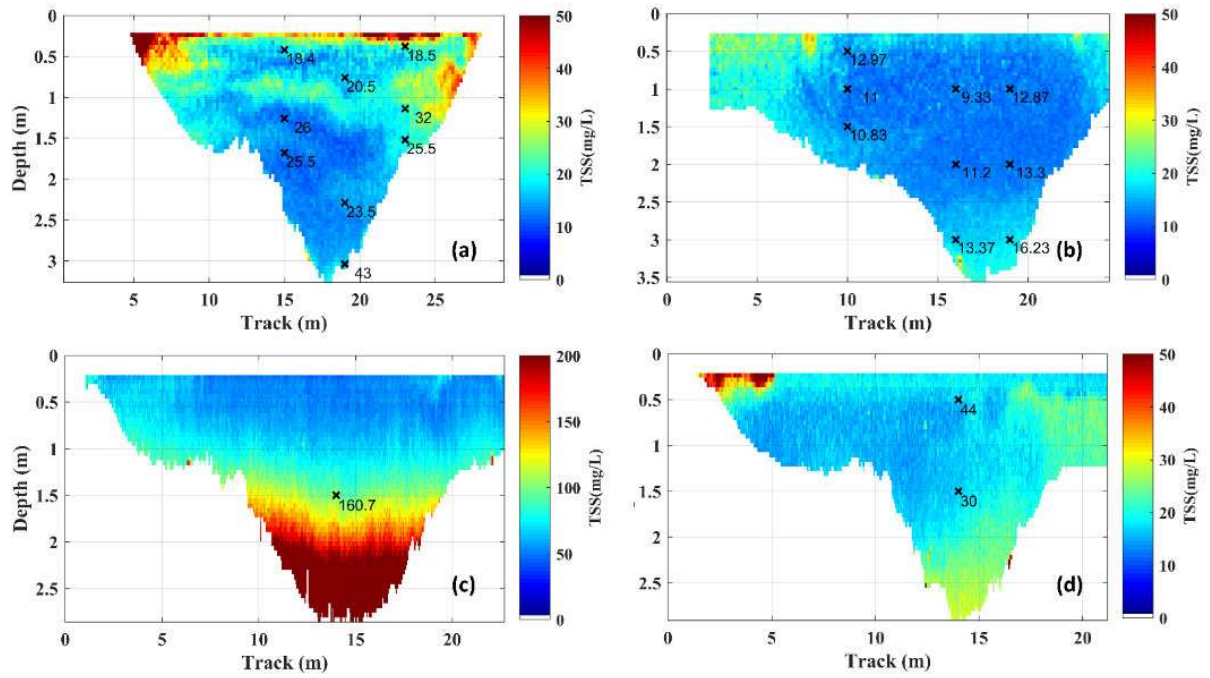
Figure 68 – Mapped cross-section in (a) Aug/17, (b) Feb/18, (c) 18Oct/18 and (d) 20Oct/18.
