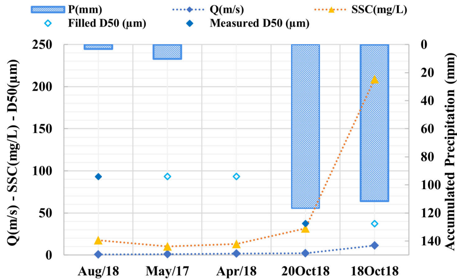
Figure 40 – Relation between the parameters obtained during the campaigns. P7 is the accumulated precipitation registered from 7 days before the measurement campaign. All parameters's values were arranged from the lowest measured discharge to the highest measured discharge.
