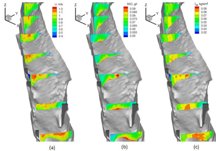
Figure 15 – Spatial distribution of a) flow velocity, b) SSC and c) Suspended Load. Adapted from: Baranya and Józsa (2013) .
