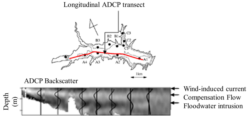
Figure 17 – Density current formation measured by Umeda, Yokoyama and Ishikawa (2006) by echosounder and ADCP measurements at Shichikashuku reservoir, in Japan.
