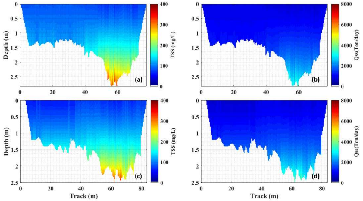
Figure 63 – Mapped cross-section in July/17 (a) TSS, (b)Qss and in August/17 (c) TSS, (d) Qss.
