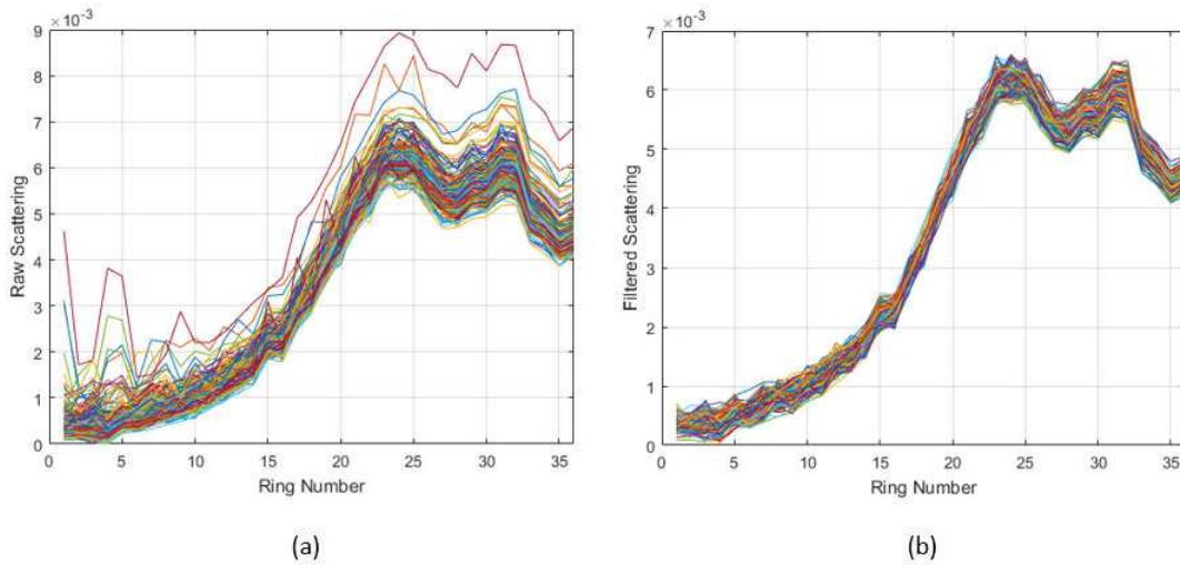
Figure 59 – Scattering Data for LISST200x (a) before and (b) after the filtering application.
