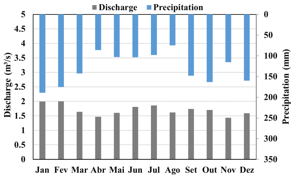
Figure 22 – Mean Precipitation and Discharge at Passauna River at Colonia Dom Pedro Station (Precipitation Data) and BR-277-Campo Largo Station (Discharge Data).
