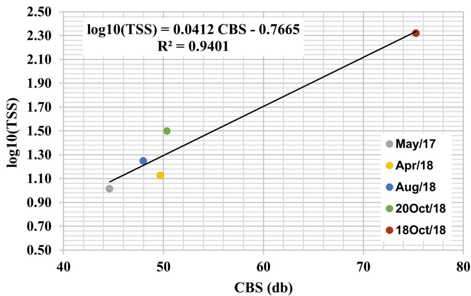
Figure 41 – Correlation curve between SSC and ADCP corrected signal at Passauna River.
