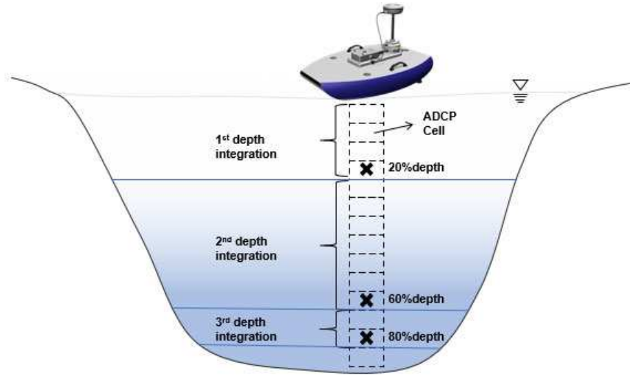
Figure 31 – Operational scheme used in the algorithm point sampling method analysis.
