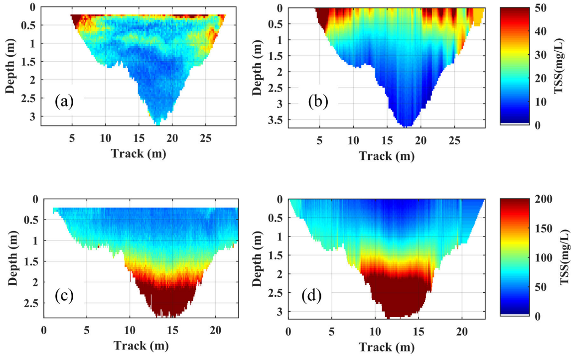
Figure 47 – Comparison between extrapolated and no-extrapolated TSS at Ferrara Bridge in Aug/17 (dry situation) and in 18Oct/18 (rainy situation).
