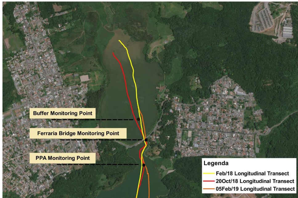
Figure 48 – Longitudinal transects and point measurements throughout the transects.
