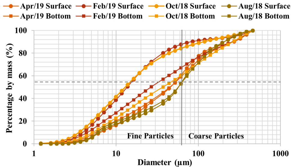
Figure 44 – Granulometric Curve at Ferrara Bridge.
