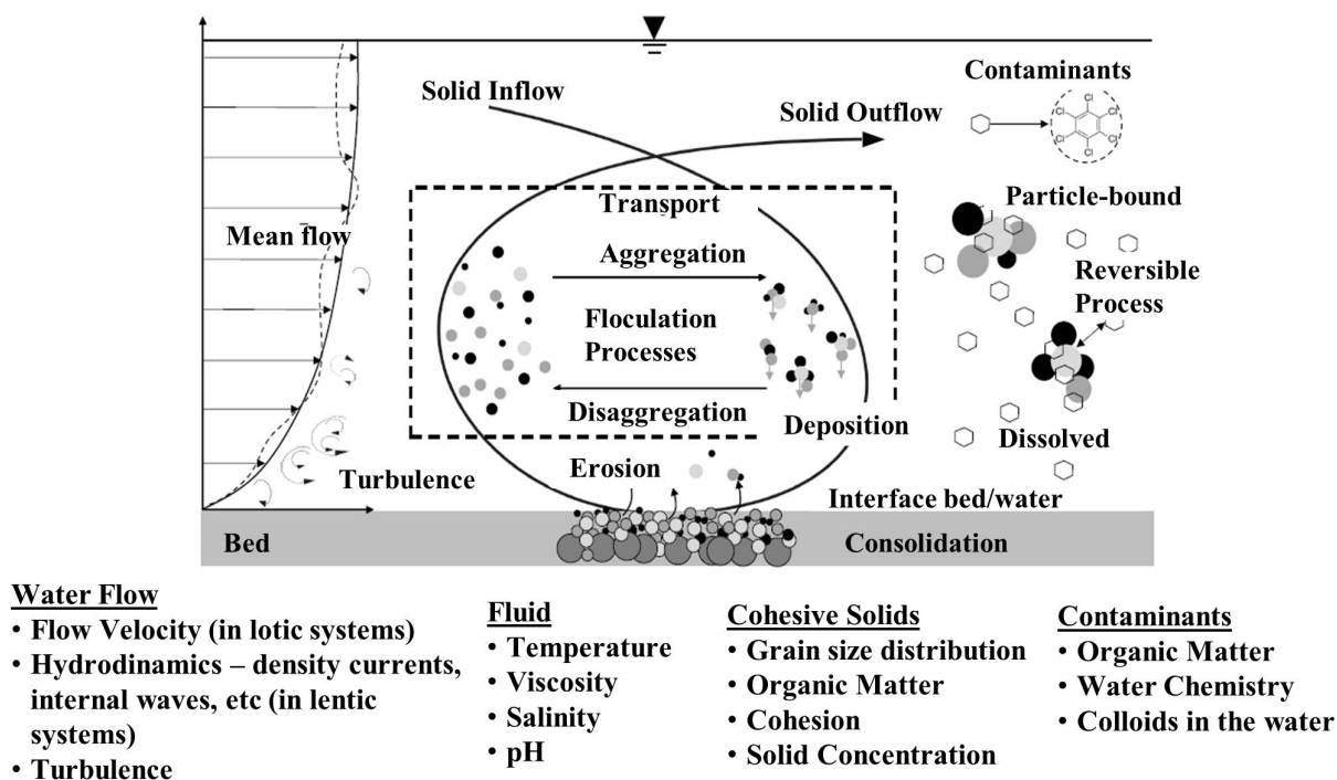
Figure 14 – Water-solid system described with a cycle of erosion, transport, deposition and consolidation, involved in particle aggregation/disaggregation and sorption/adsorption of contaminants. Below the scheme, the corresponding influence factors and the respective properties are presented.
