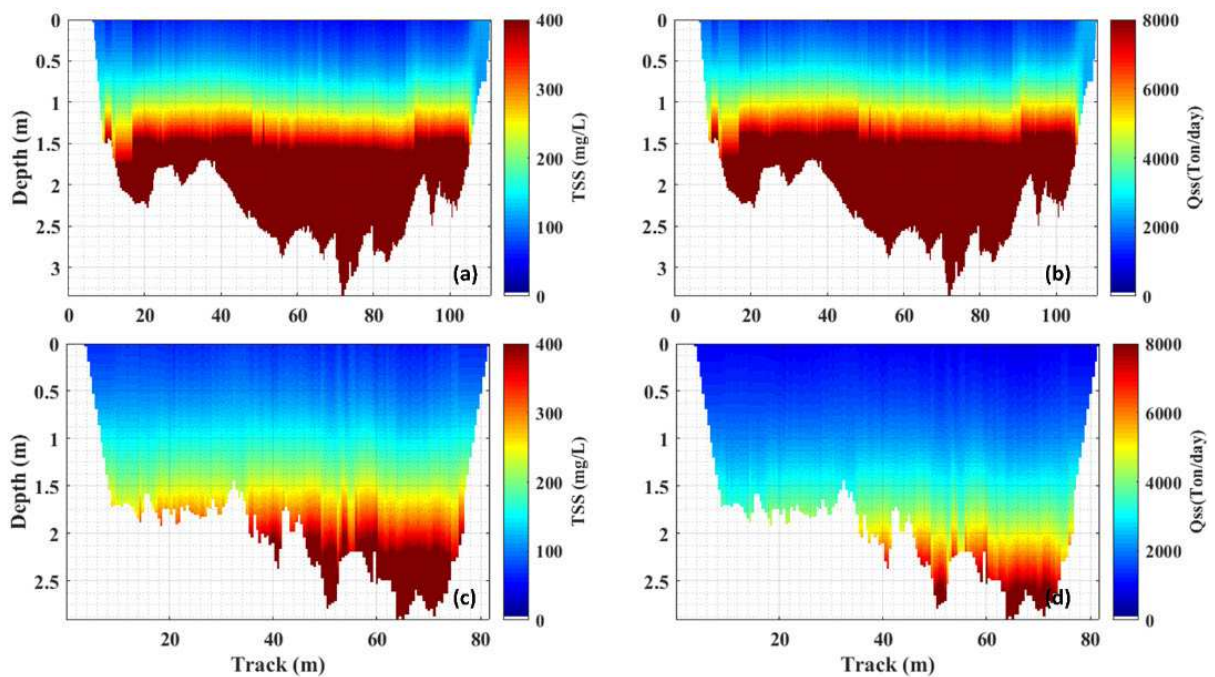
Figure 61 – Mapped cross-section in Mar/17 (a) TSS, (b)Qss and in Apr/17 (c) TSS, (d) Qss.
