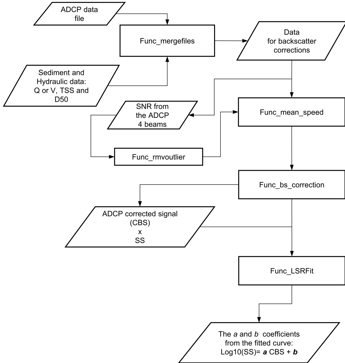
Figure 30 – Backscatter correction flowchart.
