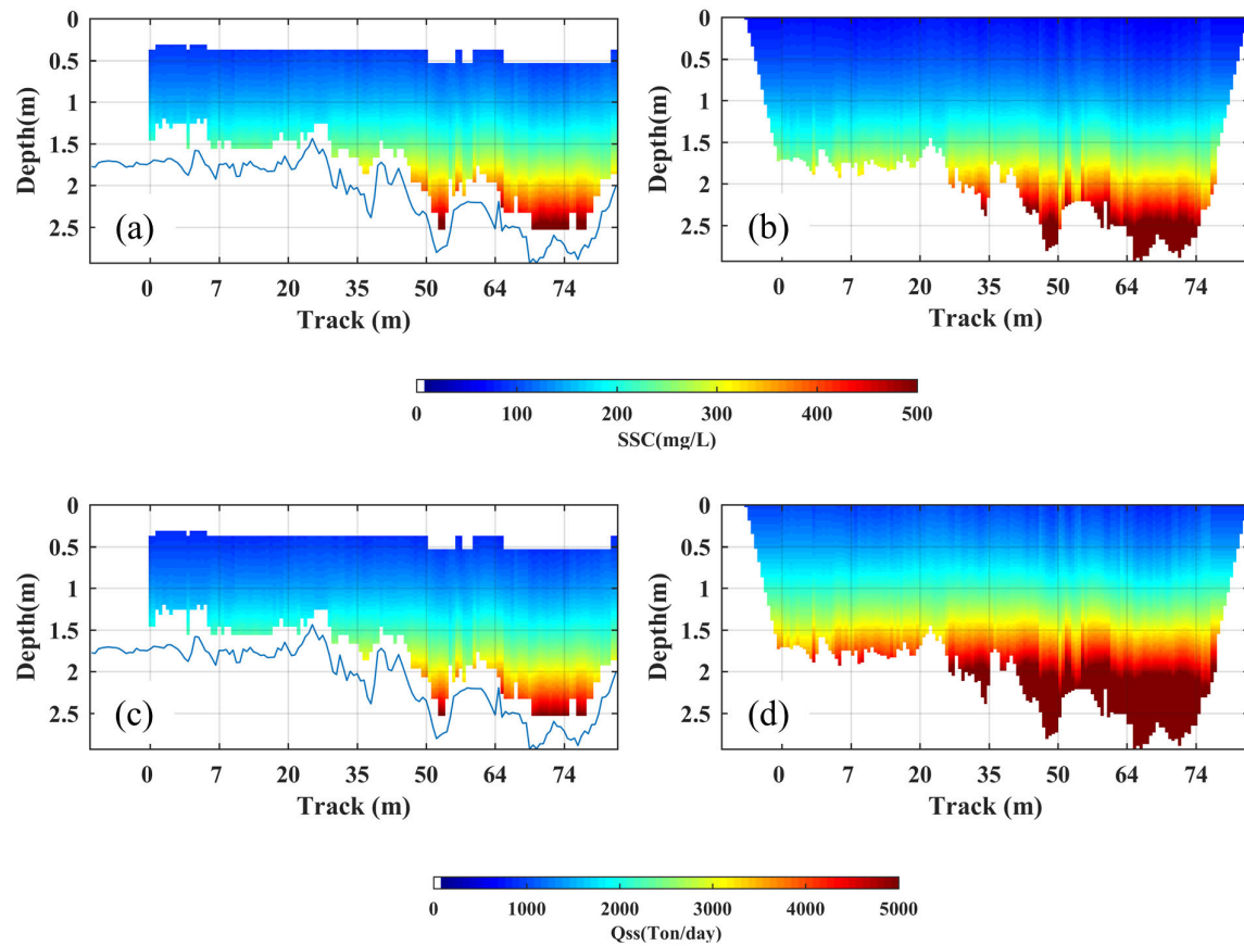
Figure 38 – Non-Extrapolated and Extrapolated Cross-Section, data from April/17: (a) Non-Extrapolated SSC, (b) Extrapolated SSC, (c) Non-Extrapolated Qss, (d) Extrapolated Qss.
