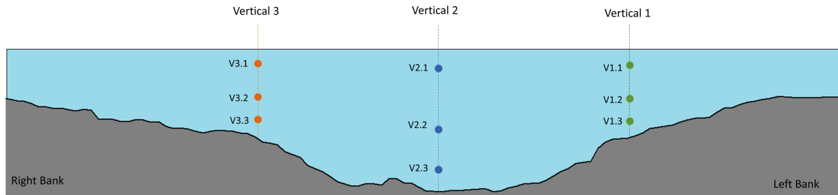
Figure 43 – Ferrara Bridge point sampling points location.
