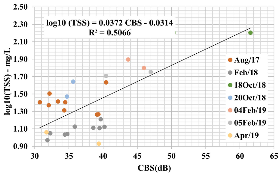
Figure 46 – Correlation curve between SSC and ADCP corrected signal at Ferrara Bridge.
