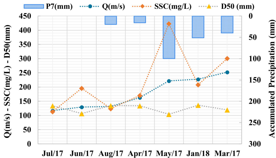
Figure 34 – Relation between the parameters obtained during the campaigns. P7 is the accumulated precipitation registered from 7 days before the measurement campaign. All parameters's values were arranged from the lowest measured discharge to the highest measured discharge.
