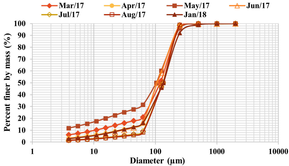
Figure 35 – Granulometric Curve for Taquari River.
