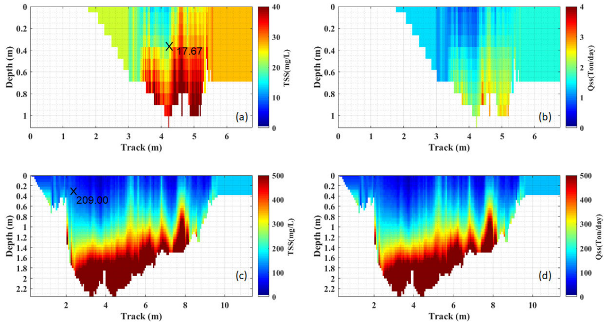
Figure 66 – Mapped cross-section in Aug/18 (a) TSS, (b)Qss and in 18Oct/18 (c) TSS, (d) Qss.
