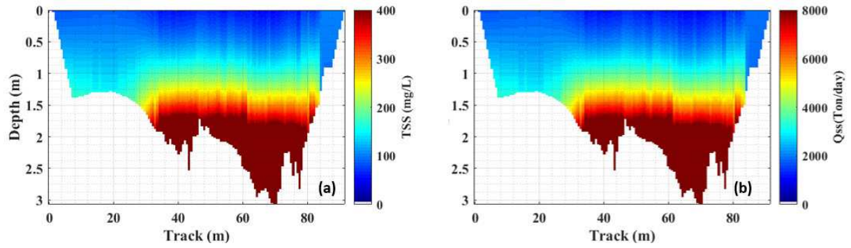
Figure 64 – Mapped cross-section in Jan/18 (a) TSS, (b)Qss.
