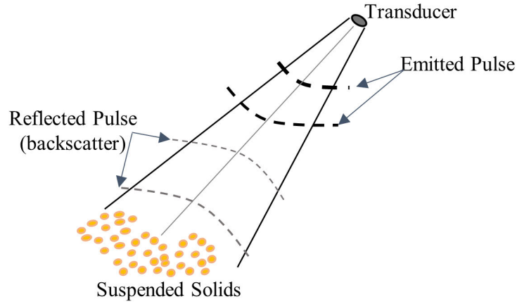
Figure 9 – Emitted pulse and reflected backscatter.
