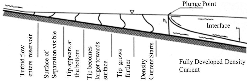
Figure 4 – Density Current Formation: a transition from non-stratified to stratified flow.
