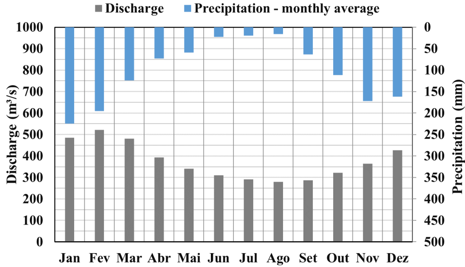
Figure 20 – Mean Precipitation and Discharge at Taquari River at Coxim Station (Code:1854004).
