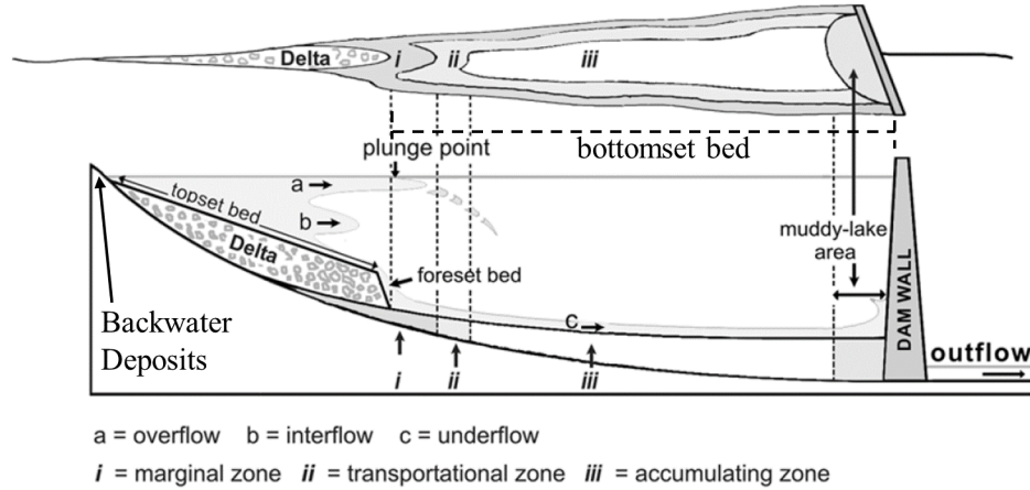
Figure 3 – Solid Deposit Formation in the transitional zone between lotic and lentic environments.
