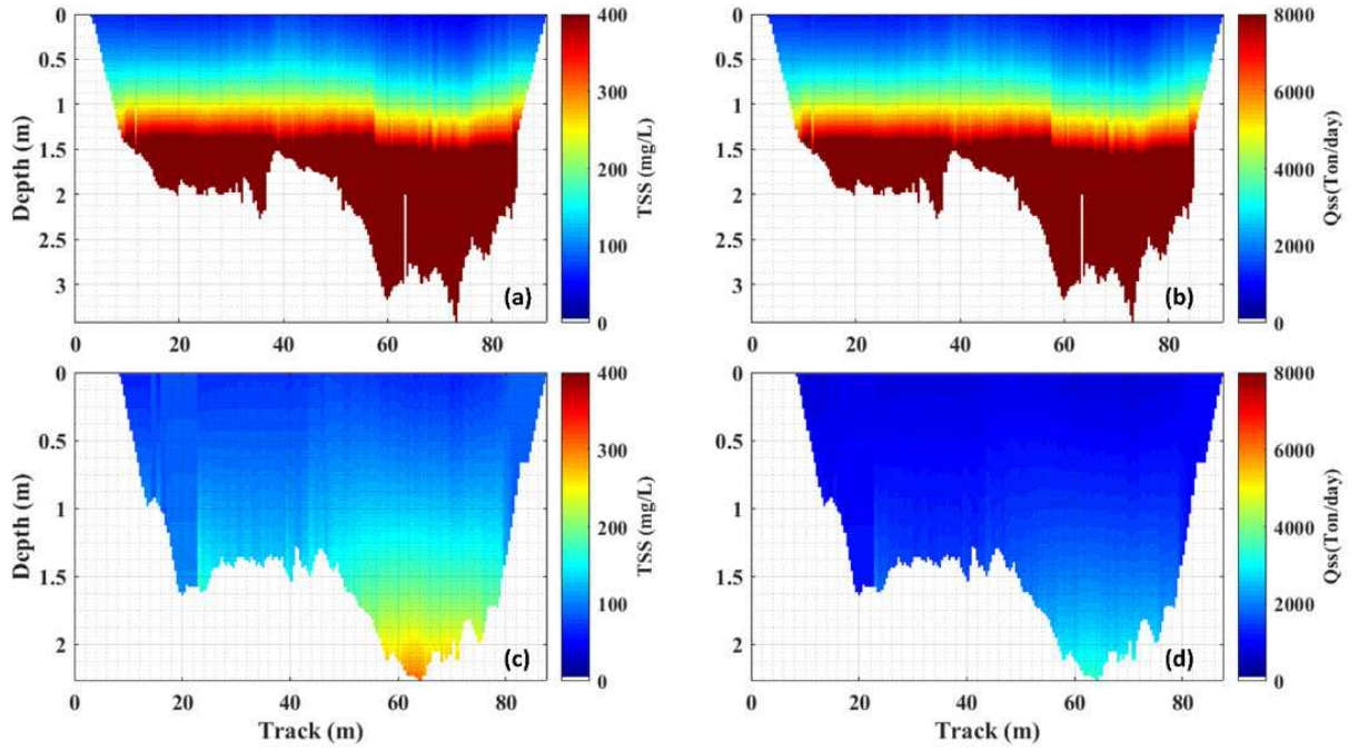
Figure 62 – Mapped cross-section in May/17 (a) TSS, (b)Qss and in June/17 (c) TSS, (d) Qss.
