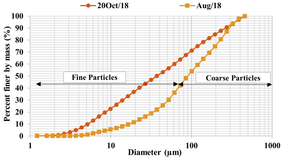
Figure 39 – Granulometric Curve for Passauna River.
