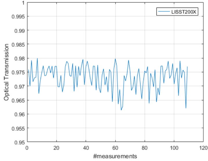
Figure 58 – Optical Transmission.
