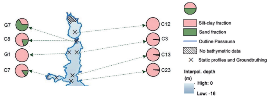
Figure 53 – Granulometry from Grab (G) and Cores (C) obtained by Sotiri, Hilgert and Fuchs (2019) at Passauna Reservoir. Adapted from: Sotiri, Hilgert and Fuchs (2019).
