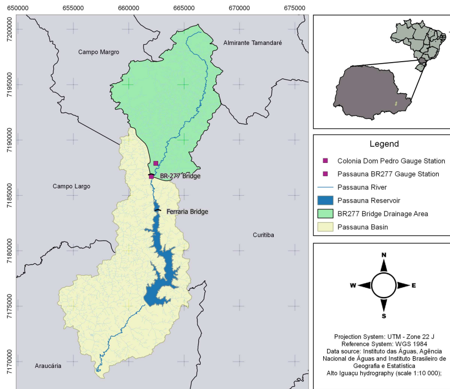
Figure 21 – Passauna Basin Location.
