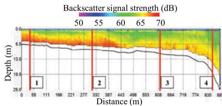
Figure 16 – Density current formation recognized by Haun and Lizano (2016) at Peñas Blancas reservoir, in Costa Rica.
