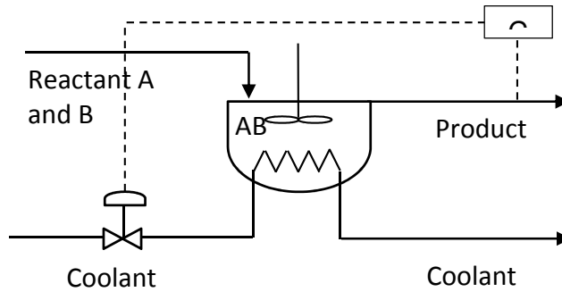
FIGURE 4-12. CONTINUOUS STIRRED TANK REACTOR
