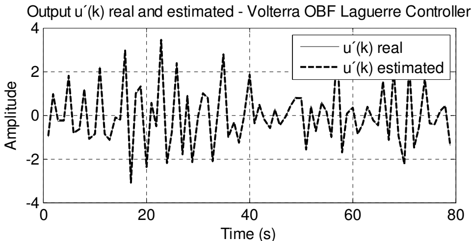
FIGURE 4-5a. ESTIMATION OF u' AND u USING VOLTERRA-LAGUERRE CLASS OF CONTROLLER, n_1, n_2 = 4 FILTERS USED.
