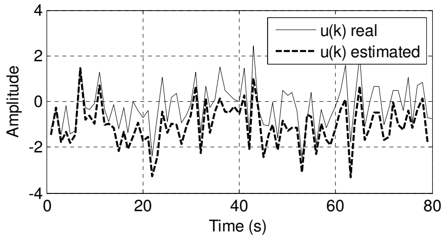
FIGURE 3-15. ESTIMATION OF u AND u' USING OBF LAGUERRE CLASS OF CONTROLLER, N = 4 FILTERS USED, NOISE WITH 0.1000 STANDARD DEVIATION.
