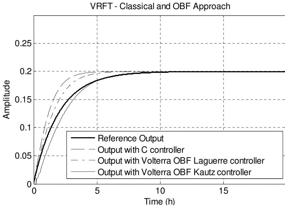
FIGURE 4-18. RESULT OF CLOSED-LOOP STEP FROM IO DATA WHEN THE CONTROLLER CLASS DOES NOT BELONG TO THE CLASS OF THE IDEAL CONTROLLER (CLASSICAL IDENTIFICATION) AND RESULT WHEN A VOLTERRA-OBF CONTROLLERS (OBF IDENTIFICATION).
