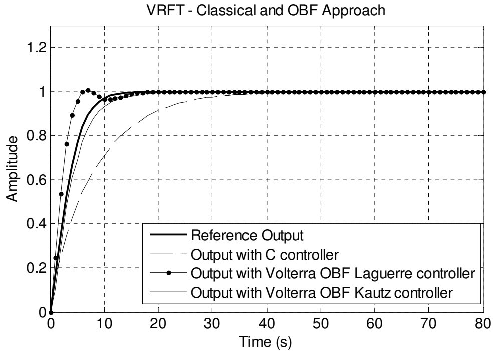
FIGURE 4-10. RESULT OF CLOSED-LOOP STEP FROM CLASSICAL IDENTIFICATION, VOLTERRA-LAGUERRE AND VOLTERRA-KAUTZ CONTROLLERS; NOISE WITH STANDARD DEVIATION 0.1.
