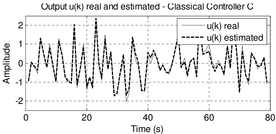
FIGURE 4-4. ESTIMATION RESULT FROM u REAL AND ESTIMATED USING CLASSICAL VRFT APPROACH WITH PRE-DEFINED CONTROL STRUCTURE.
